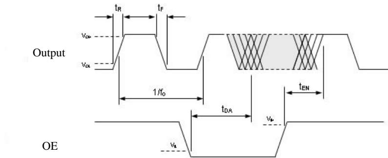
Figure 3. OE Function and Output Waveform
