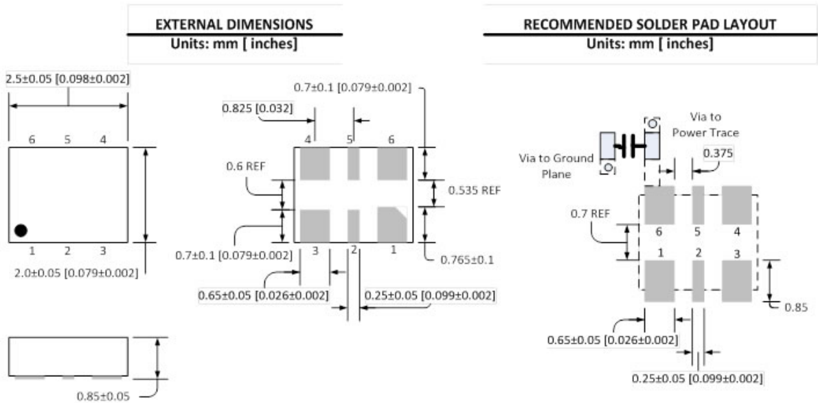
6-pin TDFN (2.5mm x 2.0mm)
