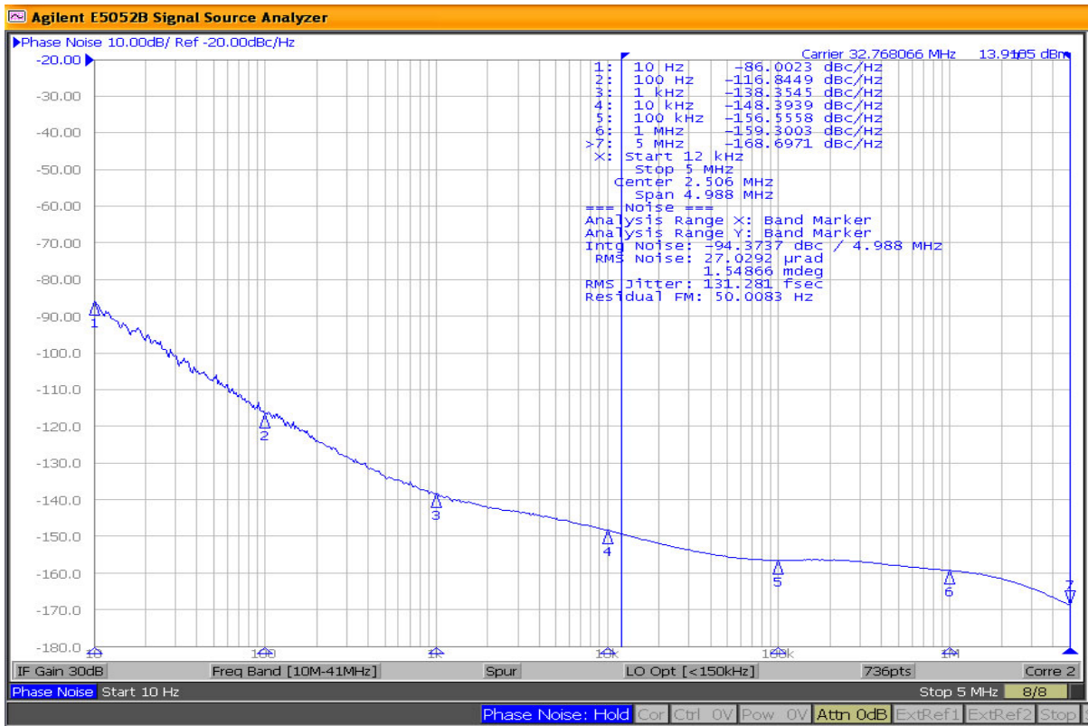
Figure 1. LVC MOS Output 32.768MHz 12kHz-5MHz 131fs
