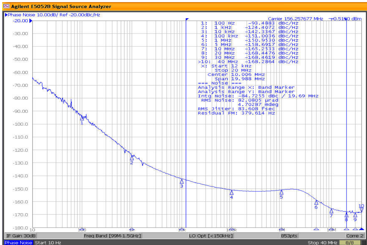
Figure 8. 156.257812MHz LVDS Output, 12kHz-20MHz 84fs
