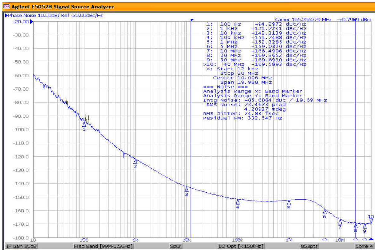
Figure 9. 156.257812MHz HCSL Output, 12kHz-20MHz 75fs
