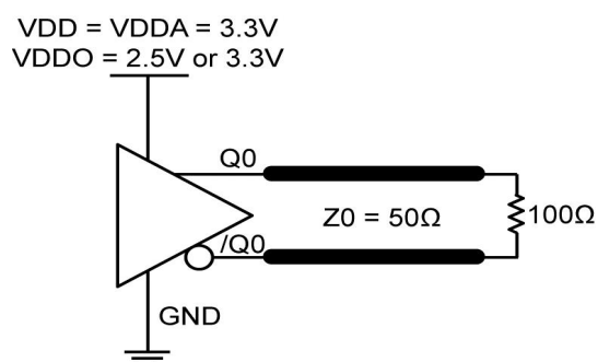
Figure 6. LVDS Output Load and Test Circuit
