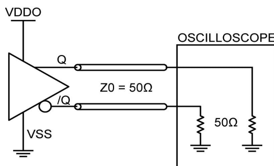
Figure 8. HCSL Output Load and Test Circuit
