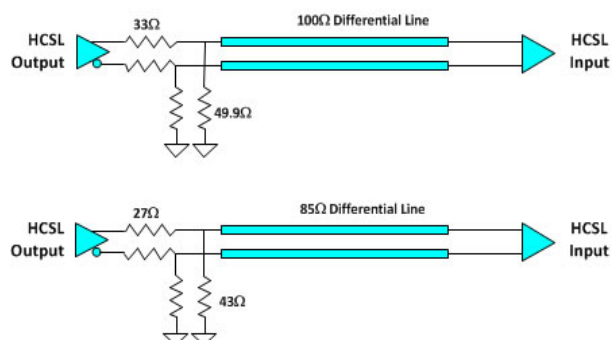
Figure 9. Recommended HCSL Output Termination Circuit
