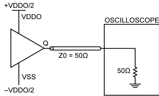
Figure 6. LVC MOS Output Load and Test Circuit
