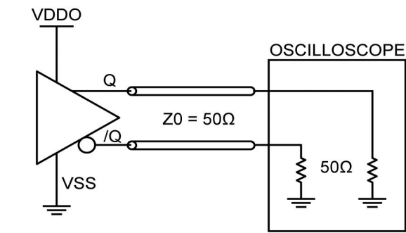
Figure 7. HCSL Output Load and Test Circuit
