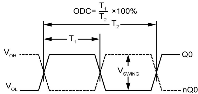
Figure 3. Duty Cycle Timing
