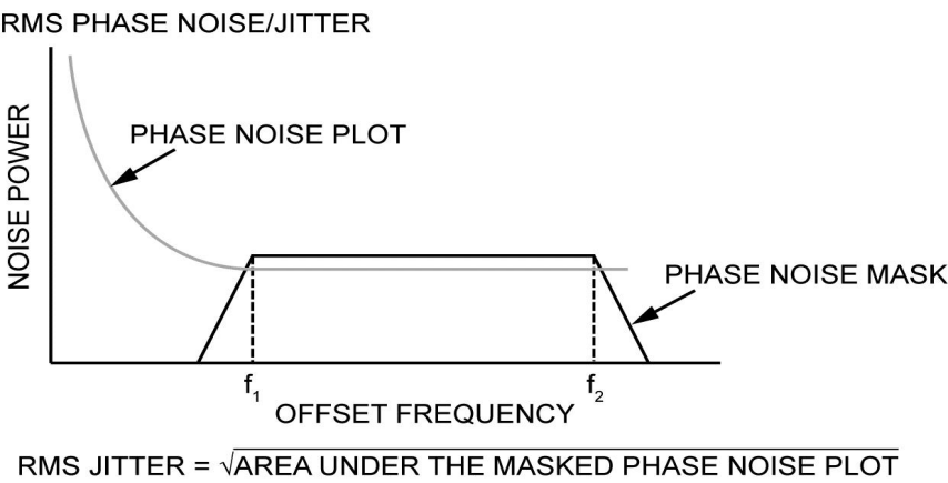
Figure 5. RMS Phase/Noise/Jitter
